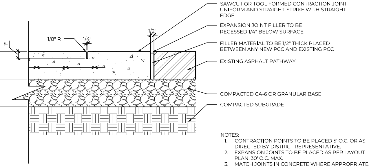
PCC BENCH PAD TO ASPHALT JOINT
