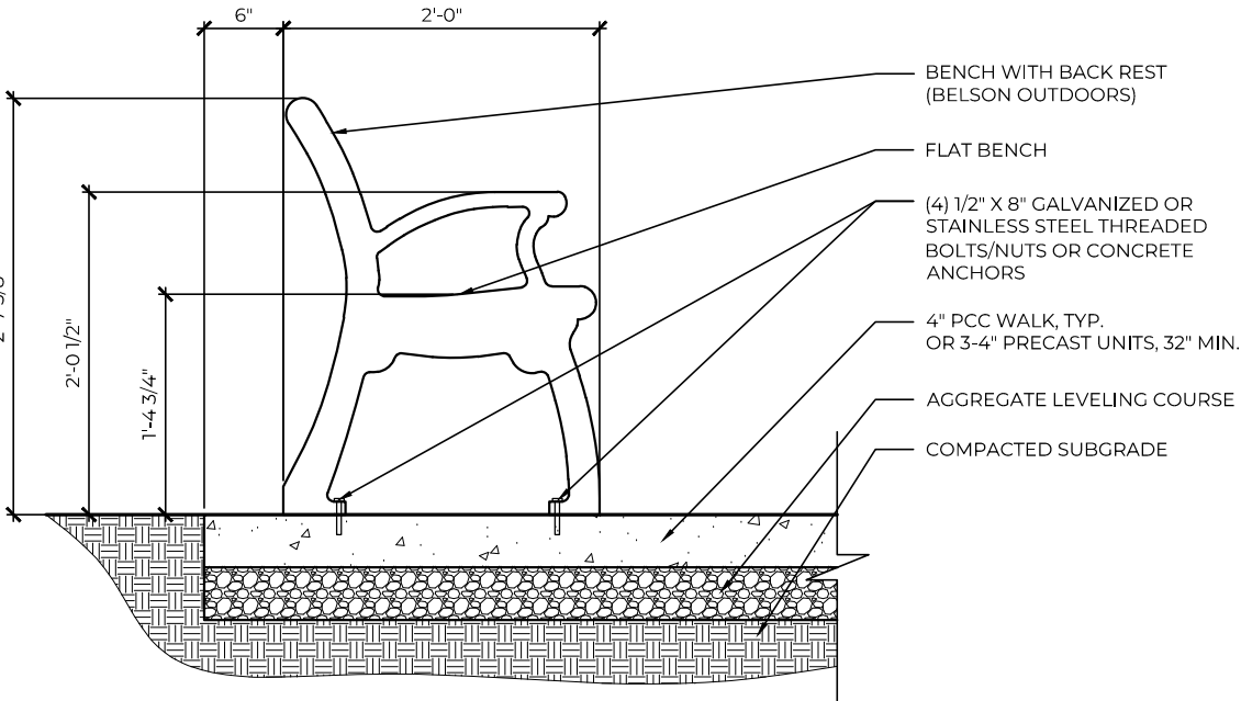
BENCH & PCC PAD SECTION
