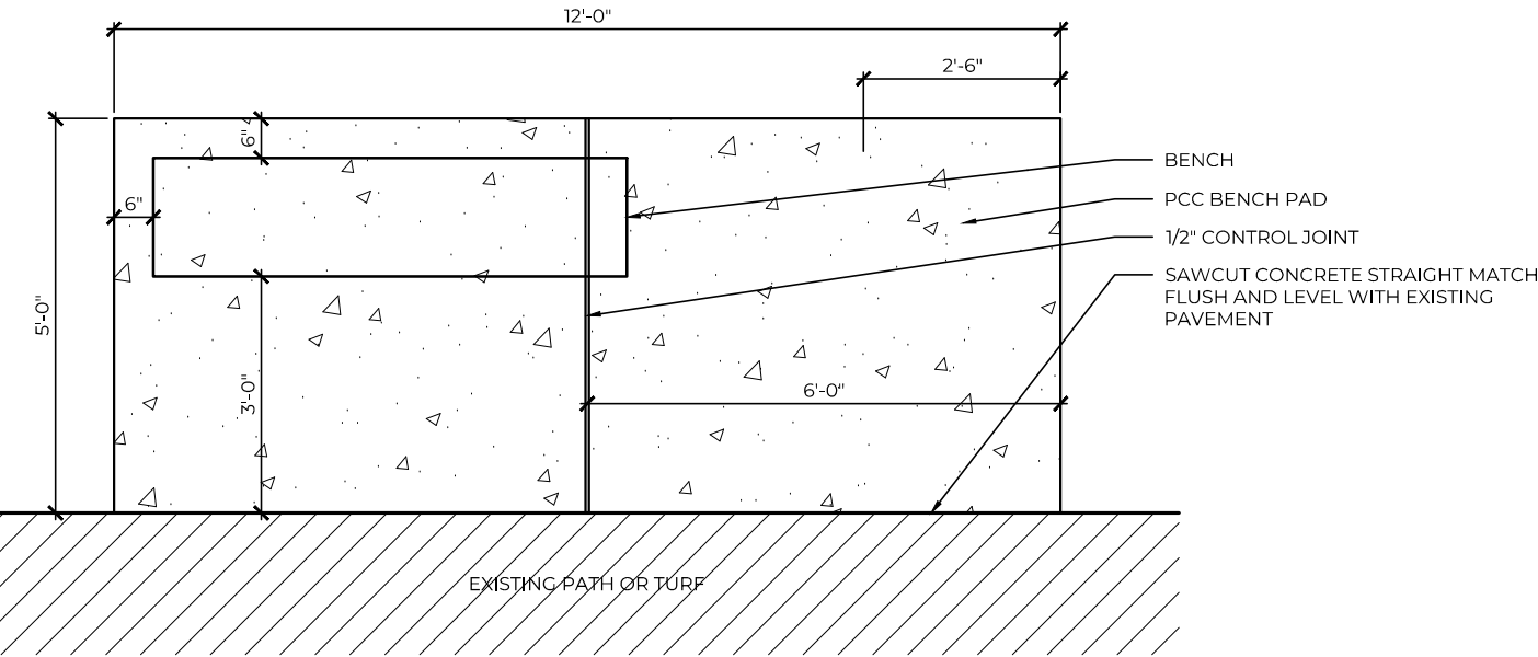
PCC BENCH PAD PLAN
